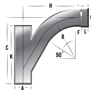
90° TY (ONE END EXPANDED)
