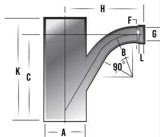
90° TY (ONE END EXPANDED)
